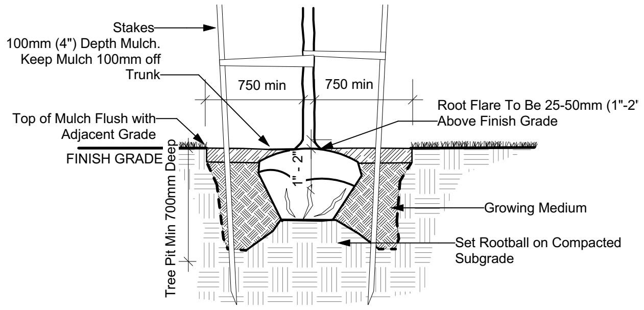
3 Tree Planting at Grade - Typical Detail Scale: 1:30
