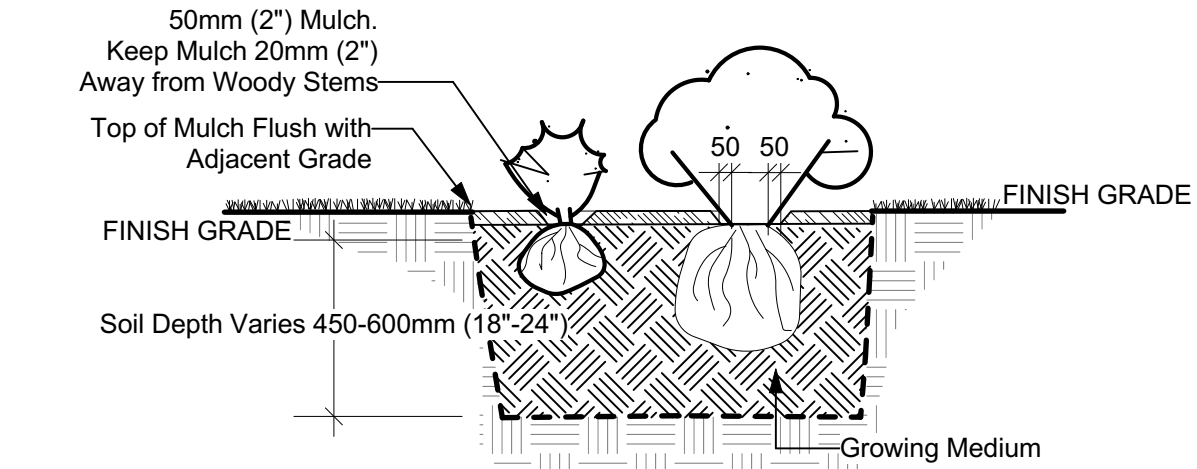
2 Shrub Planting at Grade - Typical Detail Scale: 1:30
