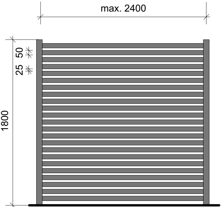
1 L1 1800mm Ht. Aluminum Privacy Screen Scale: 1:25
