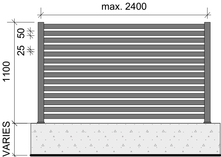
2 L1 1100mm Ht. Aluminum Fence On Planter Scale: 1:25
