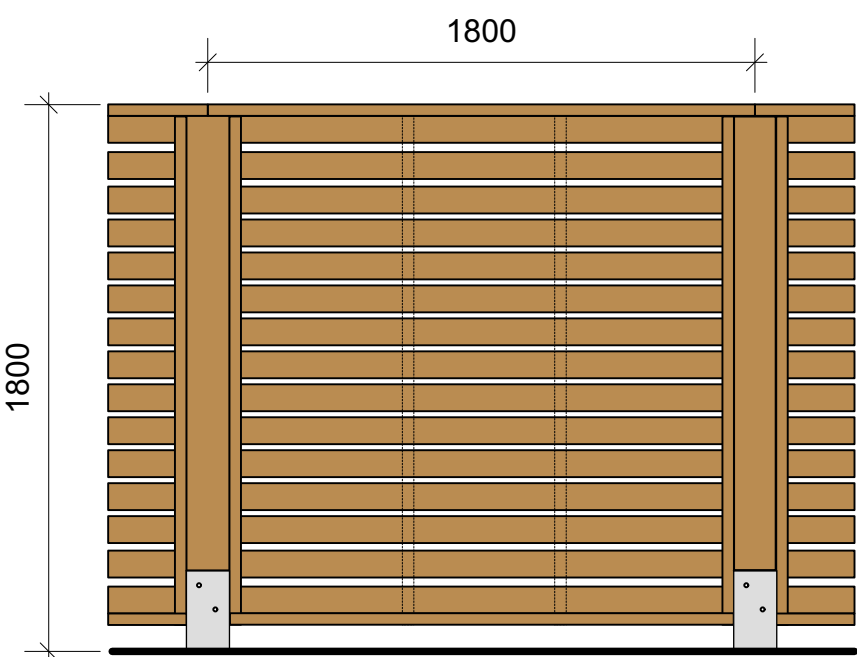
3 L1 1800mm Ht. Wood Fence Scale: 1:25
