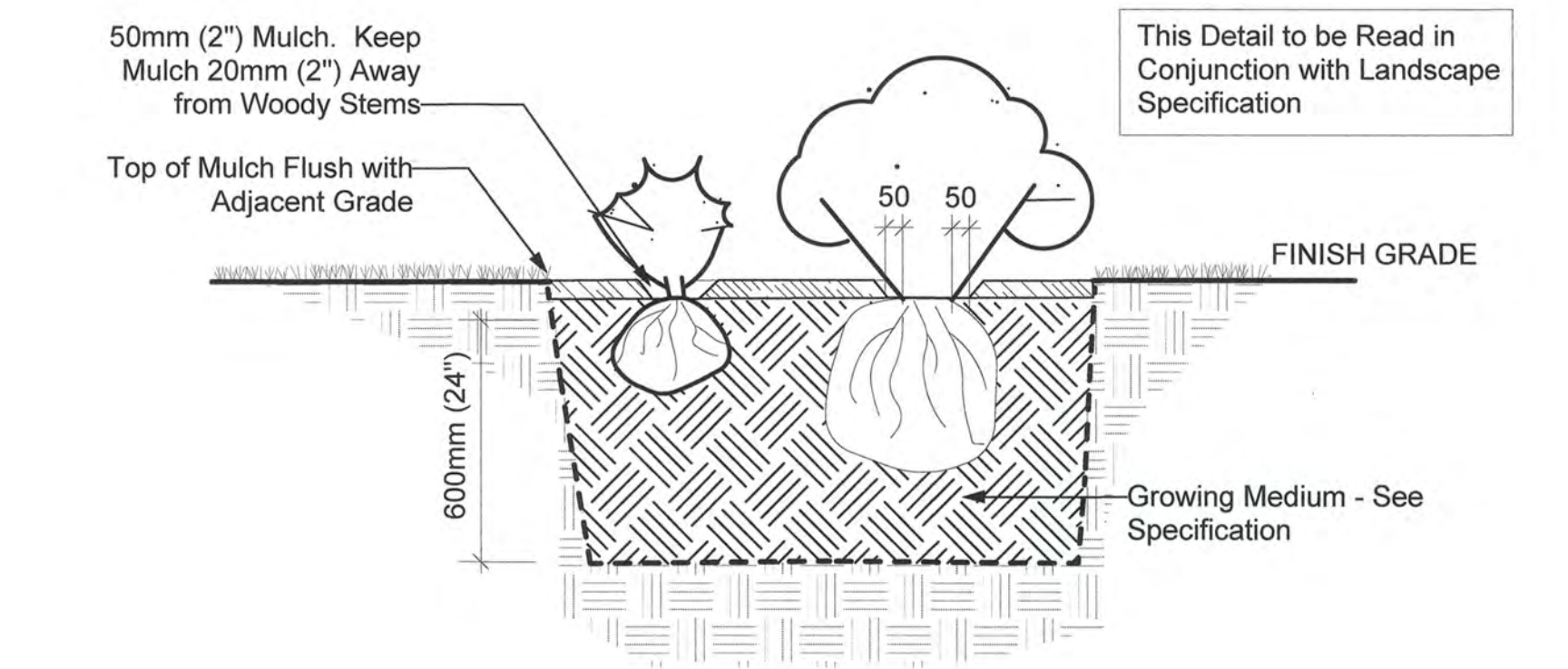
2 Shrub Planting - Typical Detail on Subgrade L10 1:20
