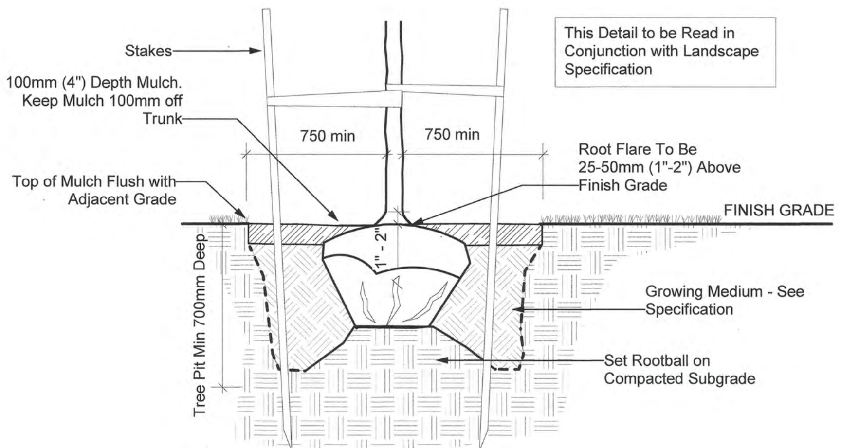
3 Tree Planting - Typical Detail on Subgrade L10 1:20
