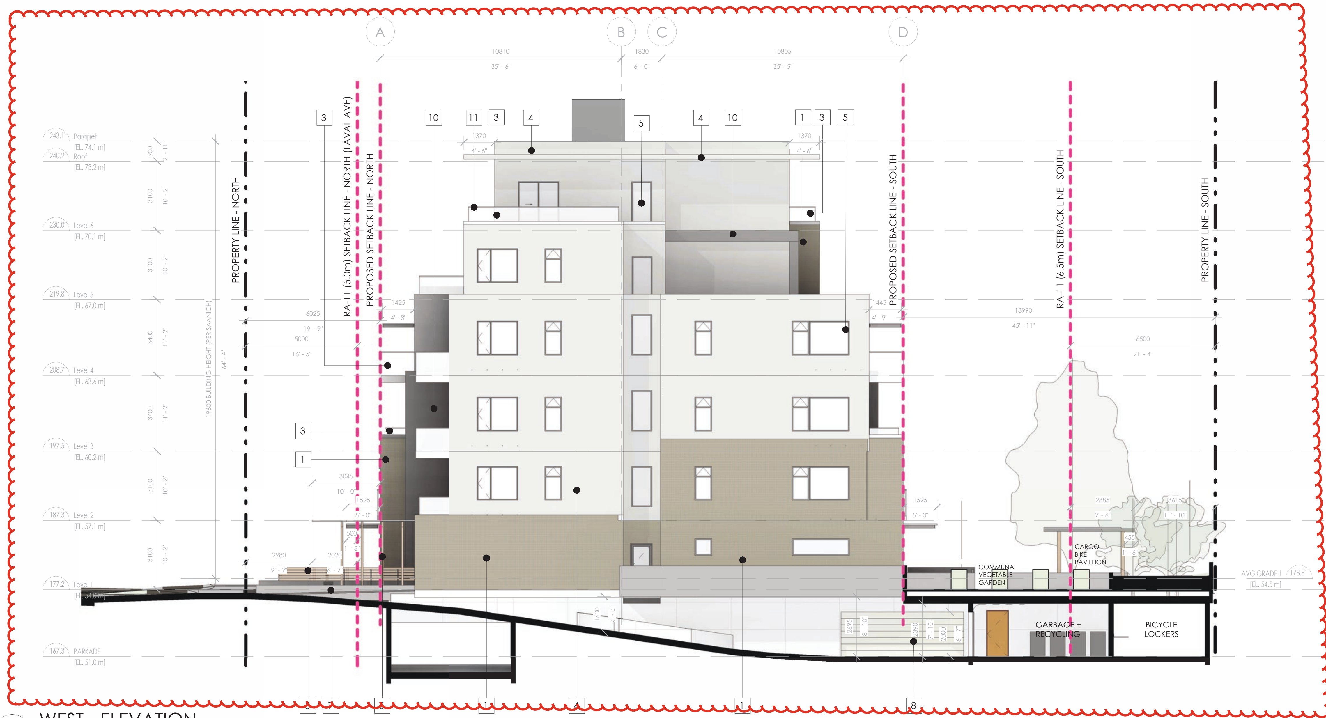
WEST - ELEVATION
