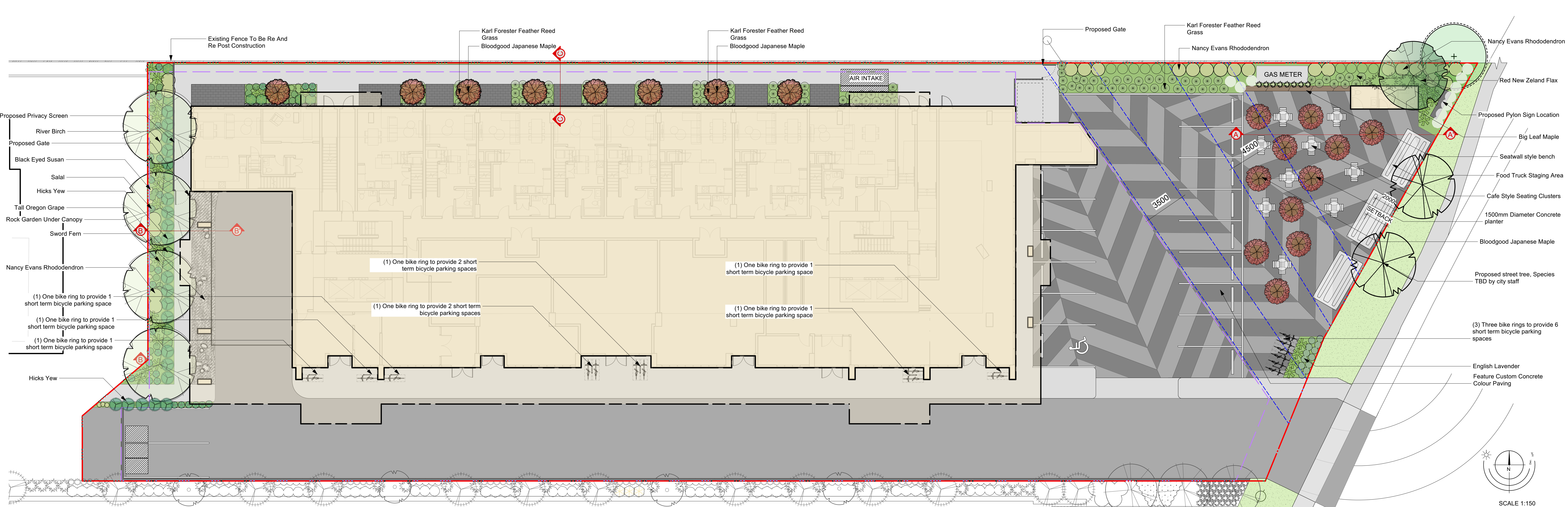
1 Landscape Concept Plan Scale 1:150
