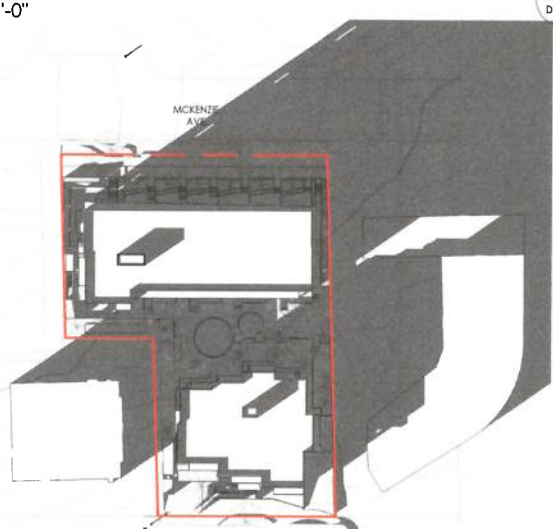
7 SUMMER SOLSTICE 3PM 1/64" = 1'-0"
