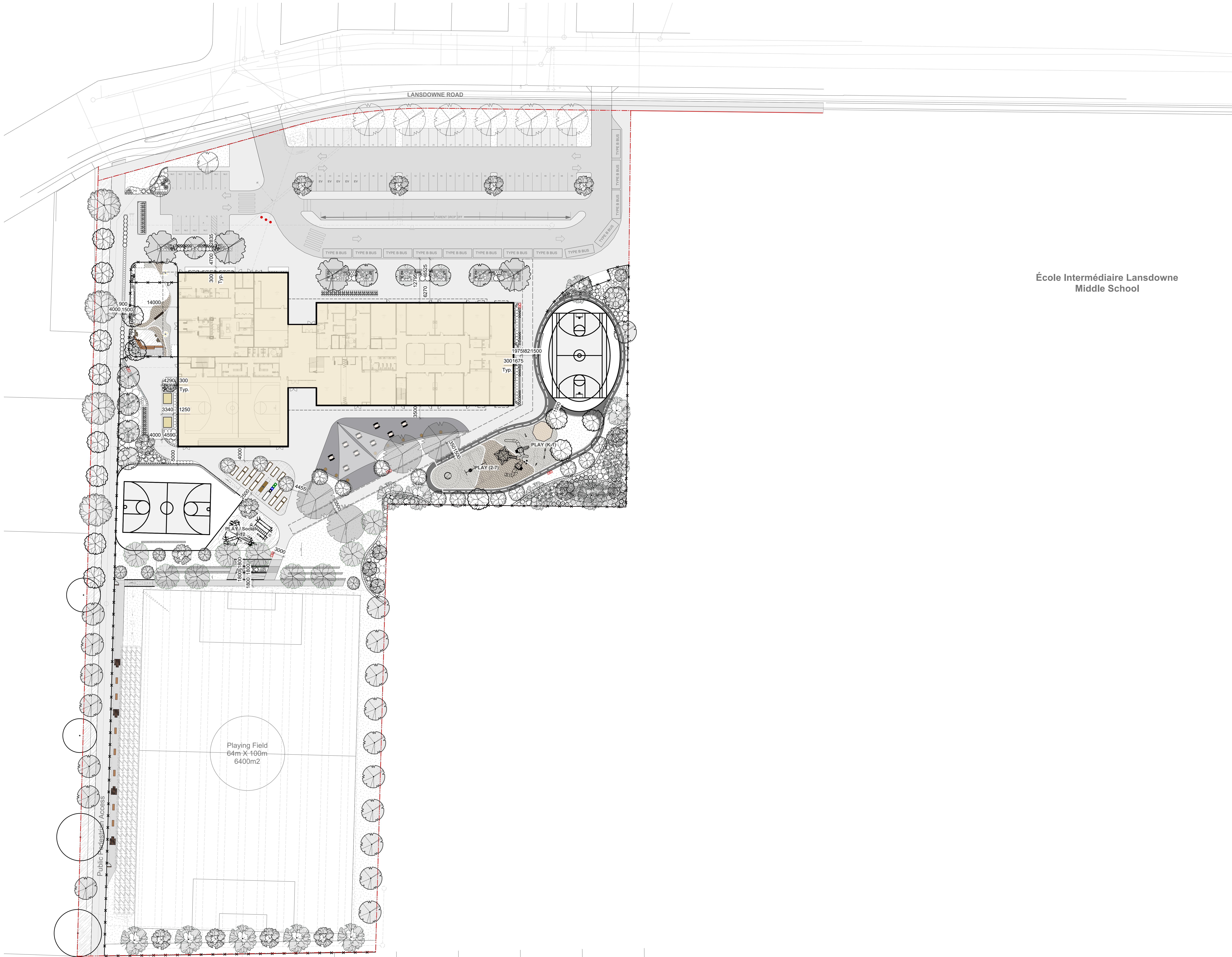
SITE LANDSCAPE PLAN - SCALE 1:350
